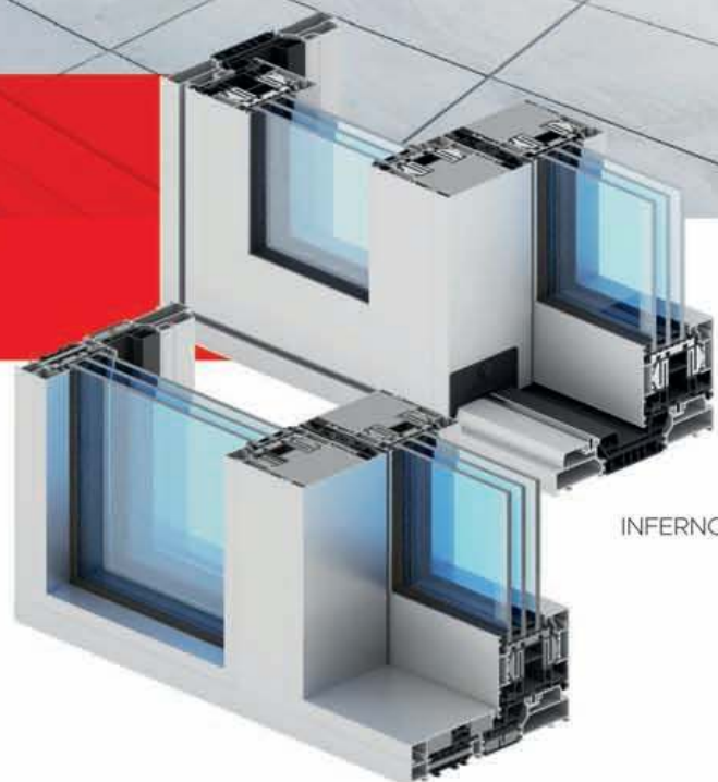
INFERNO Monorail
