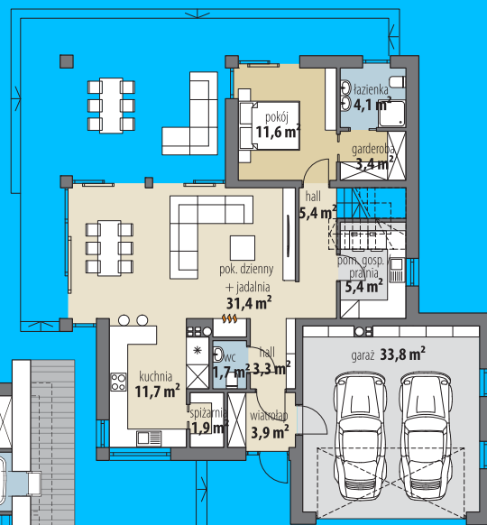
Parter
