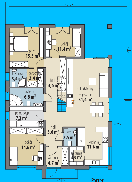
Parter
