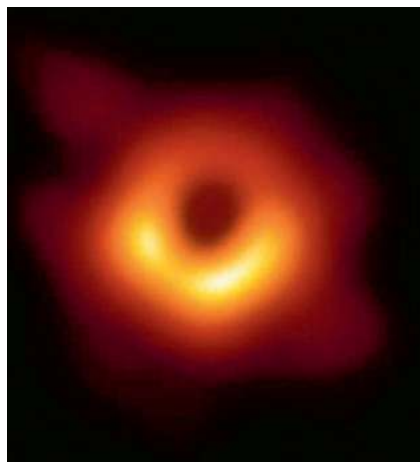
FIRST IMAGE OF A BLACK HOLE
