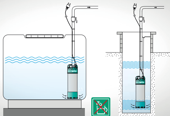
Wilo-Extract FIRST
