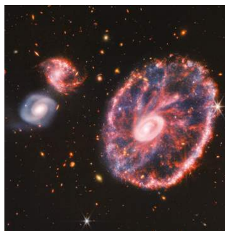
NASA/ESA/CSA/STScI/Webb ERO Production Team
